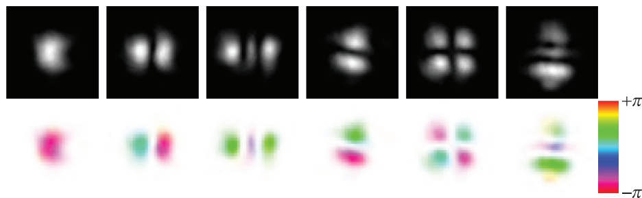
Fig. 7 Experimental results from the mode sorter. The images show intensities (top row) and phases when reading out the APVE with a Gaussian beam ( w_0 = 25 \mu\text{m} , \lambda_0 = 640 \text{ nm} ) at six different incidence angles.
