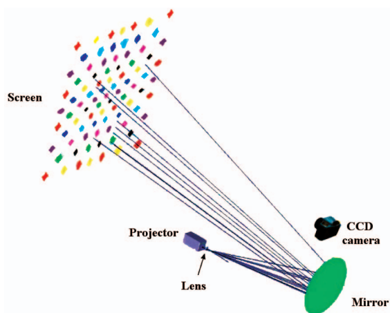
Fig. 1 Experimental setup for colored pattern projection and CCD image acquisition.
