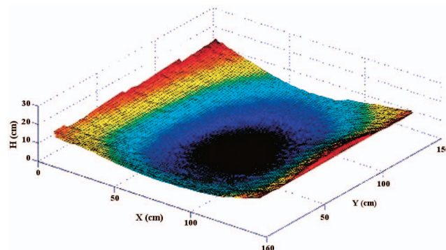
Fig. 5 A 3-D reconstruction of the mirror profile.
