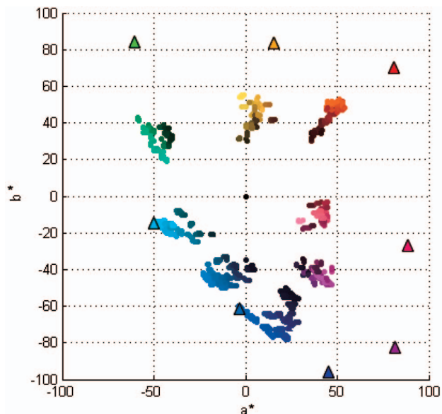
Fig. 3 Photographed colors with respect to the projected ones in the CIELAB diagram.
