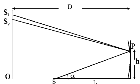
Fig. 2 Displacement between the rays reflected from the plane mirror and the curved mirror.
