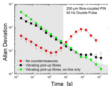
Fig. 10. Allan deviations of the pulse energy ratio of two subsequent pulses divided by the same ratio recorded with a second detector. Shown are three cases: without countermeasures against the speckle correlation, and employing vibrating pick-up fibres for the nominal on-/offline sequence and for on-line only, respectively.
