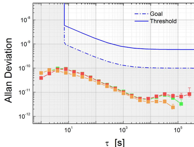
Fig. 7. Long-term relative beat-note frequency stability expressed in terms of Allan deviation for different components of the stabilized laser system: at 780 nm (green), at 1560 nm (red), and at 1557 nm (orange). See text for details. A relative value of 1 \cdot 10^{-11} corresponds to \sim 2 kHz at 1560 nm.
