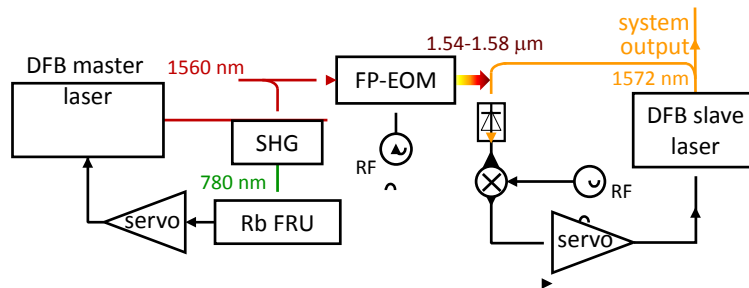
Fig. 4. Diagram of the laser system. FP-EOM: Fabry-Perot electro-optical modulator; SHG: second harmonic generation; Rb FRU: Rubidium frequency reference unit; RF: radio-frequency oscillator.
