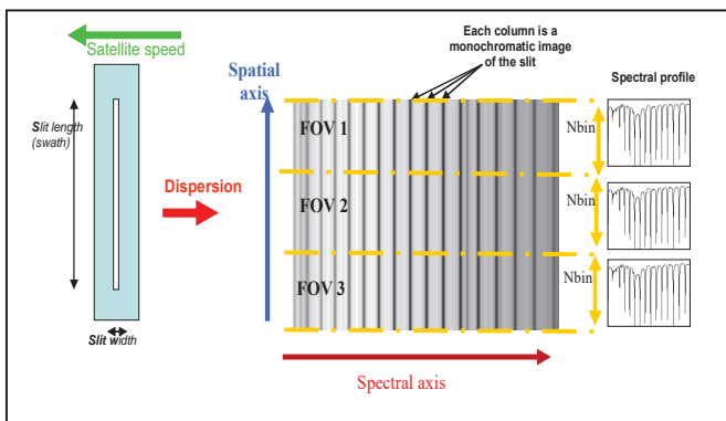
Figure 3. Illustration of spectral axis versus spatial axis
