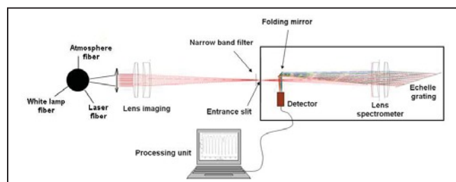
Figure 6. MicroCarb Engineering Breadboard
