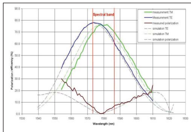
Figure 7. Comparison between grating measurement and simulation using real groove profile. 31.6 grooves/mm, Blaze = 71.45°, diffraction order 38, const deviation = 0.6°
