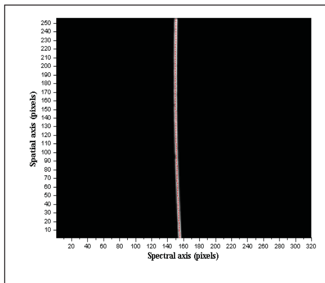
Figure 10 Estimated distortion on the image obtained using the laser
