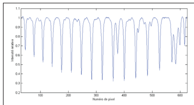
Figure 5. Example of an experiment profile for the CO 2 spectrum in band B2 (uncalibrated)
