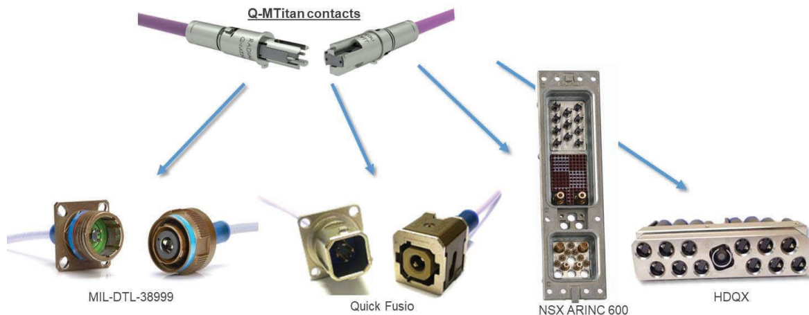
Figure 3. Q-MTitan™ fits various interconnect solutions
