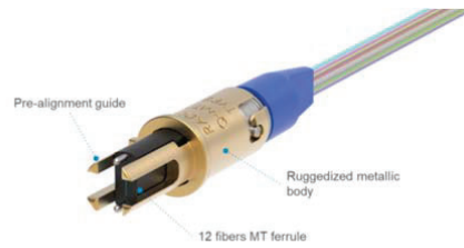
Figure 4. Q-MTitan™ ARINC 846 Aerospace industry standard for multi-fiber contact
