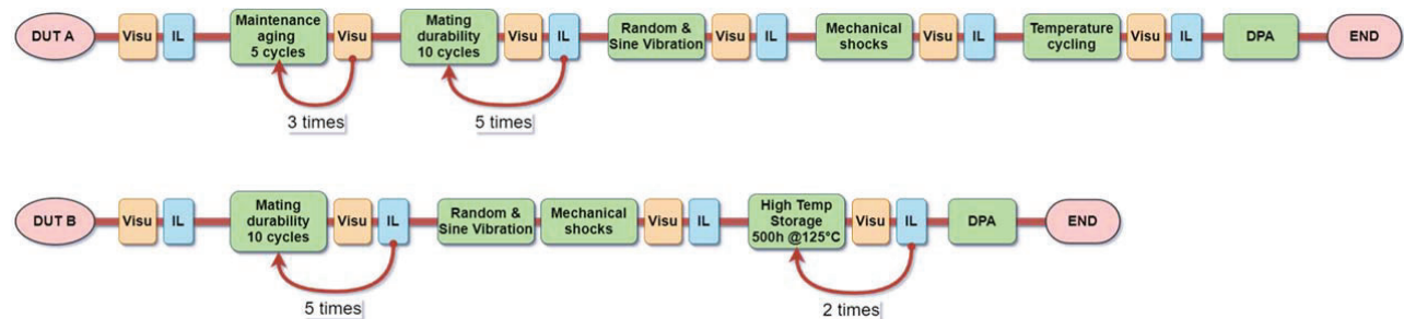
Figure 8. Test plan with 2 files of tests
