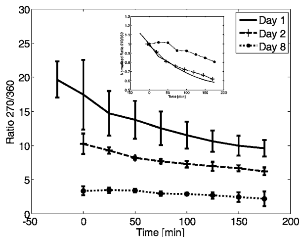
Fig. 4 Time-dependent fluorescence changes in collagen gels based on a ratio of decreasing fluorescence ( \lambda_{ex}=270 nm) to increasing fluorescence ( \lambda_{ex}=360 nm). The largest signal changes occur in the first two days with overall decrease observed out to day 8. Error bars represent the standard deviation of the data ( n=5 for day 1, n=3.4 for days 2 and 8). Inset: Normalized mean ratio for comparison of slope between groups with the greatest decrease over time at day 1 and a decrease in slope or fluorescence variation by day 8.
