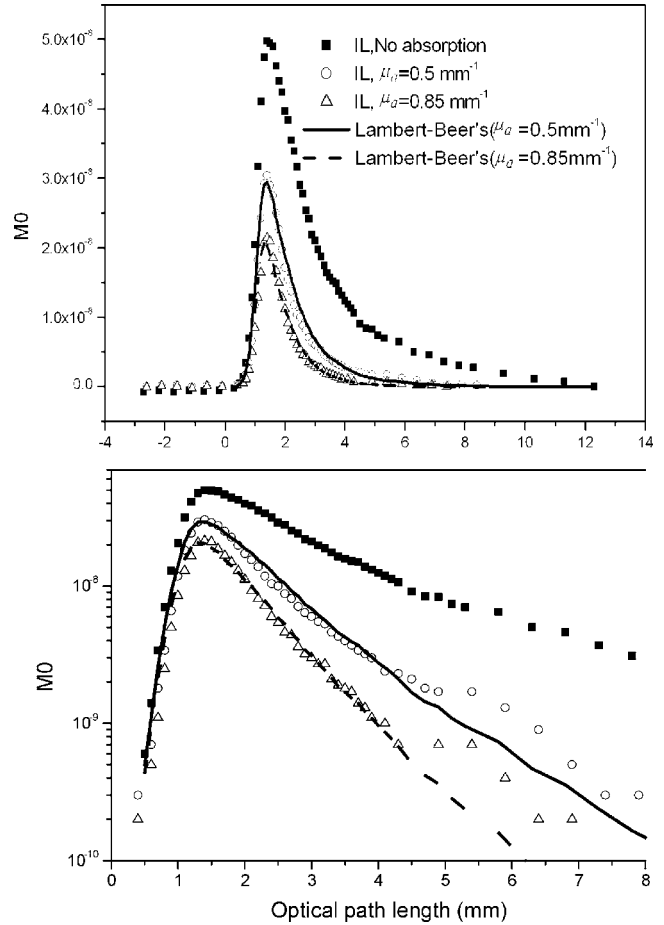
Fig. 4 Optical path length distributions estimated from the zero-order moment of the phase modulation peak for an aqueous Intralipid suspension ( \mu_a=0.001 \text{ mm}^{-1} ) and for identical suspensions with two different absorption coefficients (0.50 and 0.85 \text{ mm}^{-1} ), but equal reduced scattering coefficient (linear and logarithmic scales). The lines result from the application of Lambert-Beer's law on the experimental dataset for zero absorption.
