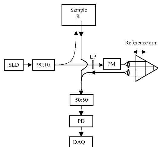
Fig. 2 Schematic of the fiber optic Mach-Zehnder interferometer. Single-mode and gradient-index multimode fibers are shown by thin and thick lines, respectively. SLD denotes superluminescent diode, PD is the photodetector, LP is a linear polarizer, PM is the electrooptic phase modulator, and 90:10 and 50:50 are single-mode and multimode fiber couplers, respectively.
