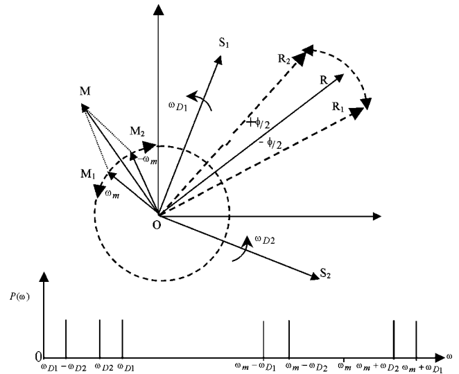
Fig. 1 Phasor diagram for the interfering fields (top) and the resulting power spectrum (bottom).
