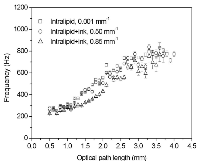
Fig. 5 The average Doppler shift extracted from the phase modulation peak as a function of the optical path length for an aqueous Intralipid suspension ( \mu_a=0.001 \text{ mm}^{-1} ) and for identical suspensions with two different absorption coefficients (0.50 and 0.85 \text{ mm}^{-1} ).
