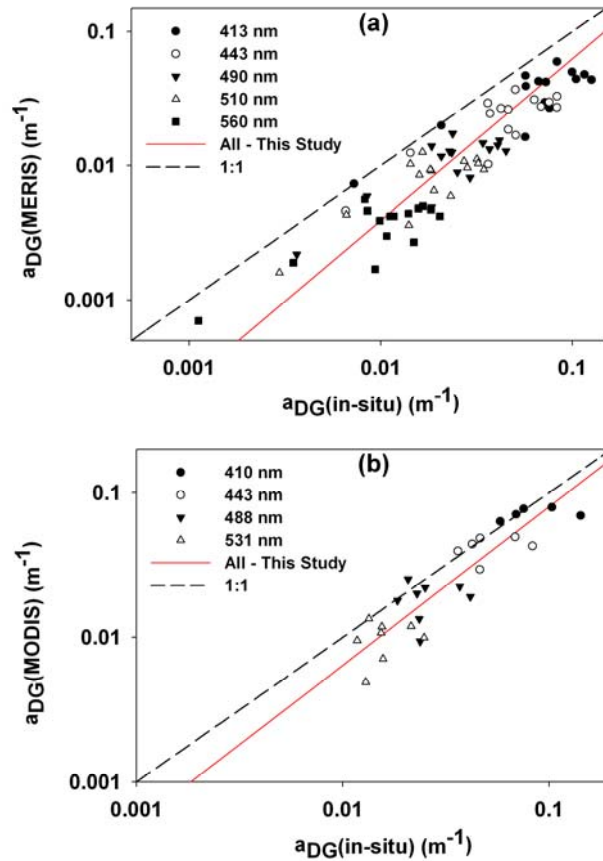
Fig. 9. Relationship between log-transformed in-situ a_{DG}(\lambda) versus QAA retrieved (a) MERIS a_{DG}(\lambda) , and (b) MODIS a_{DG}(\lambda) . Statistics of the linear fit for each wavelength are shown in Table 3.
