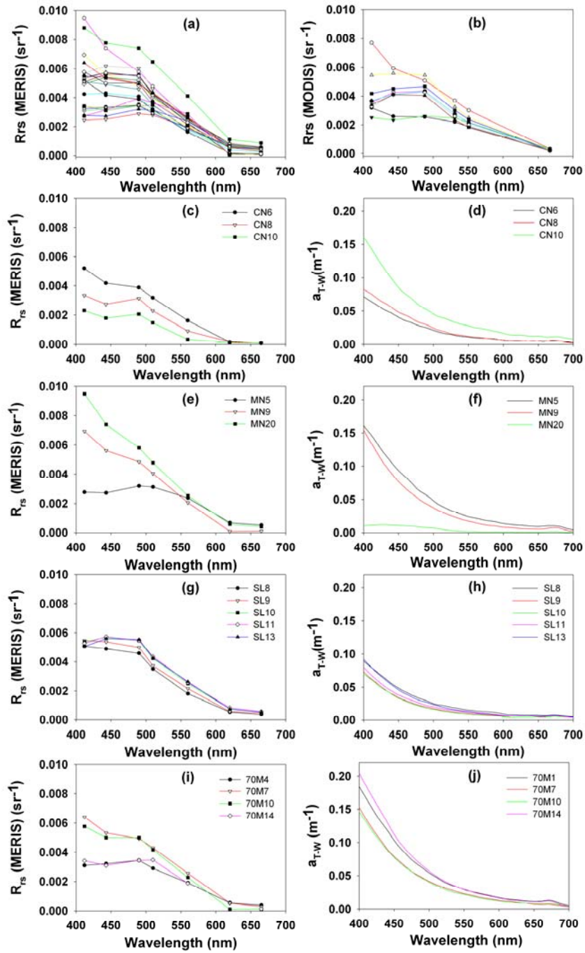
Fig. 5. Remote Sensing reflectance spectra ( R_{rs}(\lambda) ) from (a) MERIS, and (b) MODIS ocean color sensors. Comparison of MERIS R_{rs}(\lambda) and in-situ a_{T,W}(\lambda) for (c-d) CN transect, (e-f) MN transect, (g-h) SL transect, and (i-j) 70M transect. Transect and station locations are shown in Fig. 1.
