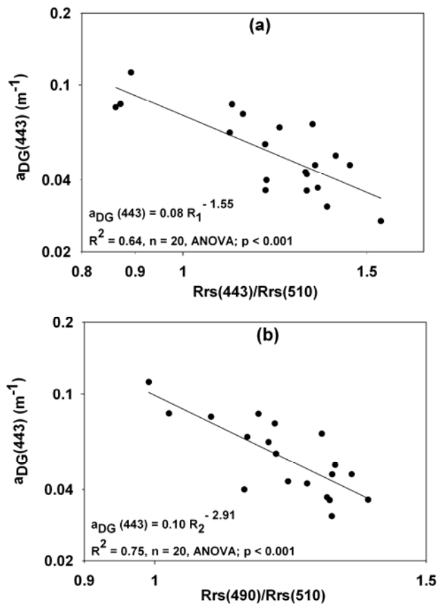
Fig. 7. Relationships between a_{DG}(\lambda) at 443 nm and the blue-to-green ratio of R_{rs}(\lambda) . (a) a_{DG}(443) versus R_{rs}(443)/R_{rs}(510) ( R_1 ), and (b) a_{DG}(443) versus R_{rs}(490)/R_{rs}(510) ( R_2 ). The least squares fit (solid lines and equations), the R^2 for log-transformed data, and the number of observations ( n ) are shown.
