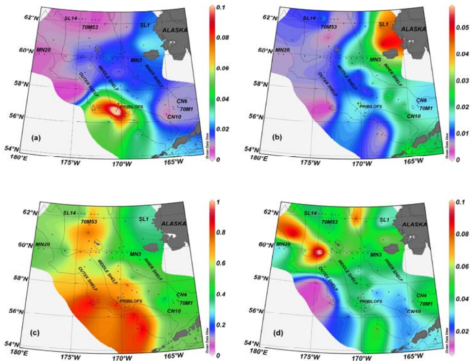
Fig. 2. Surface distribution of (a) phytoplankton absorption, a_{PHY}(443) ( \text{m}^{-1} ) (b) Non-algal/detrital absorption, a_{NAP}(443) ( \text{m}^{-1} ), (c) ratio of phytoplankton and total particulate absorption, a_{PHY}(443)/a_P(443) and (d) chlorophyll-a specific phytoplankton absorption, a^*_{PHY}(443) ( \text{m}^2 (\text{mg chl } a)^{-1} ) at 443 nm.
