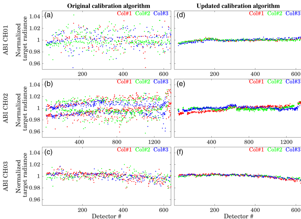
Fig. 18 Detector-uniformity analysis with normalized mean-radiance NL_{c,k} (%) among detectors of column c ( c = 1, 2, and 3 ) for ABI CH01 to CH03 as derived from (a–c) version O and (d–f) version U calibration algorithms.
