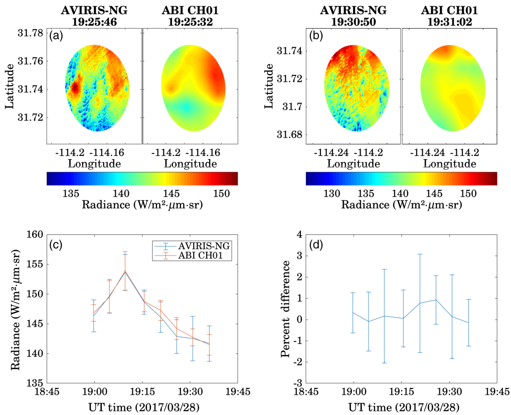
Fig. 5 (a) and (b) Selected comparison between sampled GOES-16 ABI MESO and AVIRIS-NG data over two ray-matching sites ( <5 deg) during March 28, 2017, for ABI CH01. The AVIRIS-NG data were convolved with the SRF of ABI CH01. ABI MESO data was sampled into the 5-deg ray-matching region. (c) Time series of mean radiance over the ray-matching sites derived from GOES-16 ABI MESO and AVIRIS-NG measurements for ABI CH01. Vertical bars indicate the standard deviation of scene radiance due to scene nonuniformity. (d) Time series of percent difference between the mean radiances of ABI and AVIRIS-NG over the ray-matching sites for ABI CH01. The error bars mark the one-sigma standard deviation ( k = 1 ) of the percent differences.
